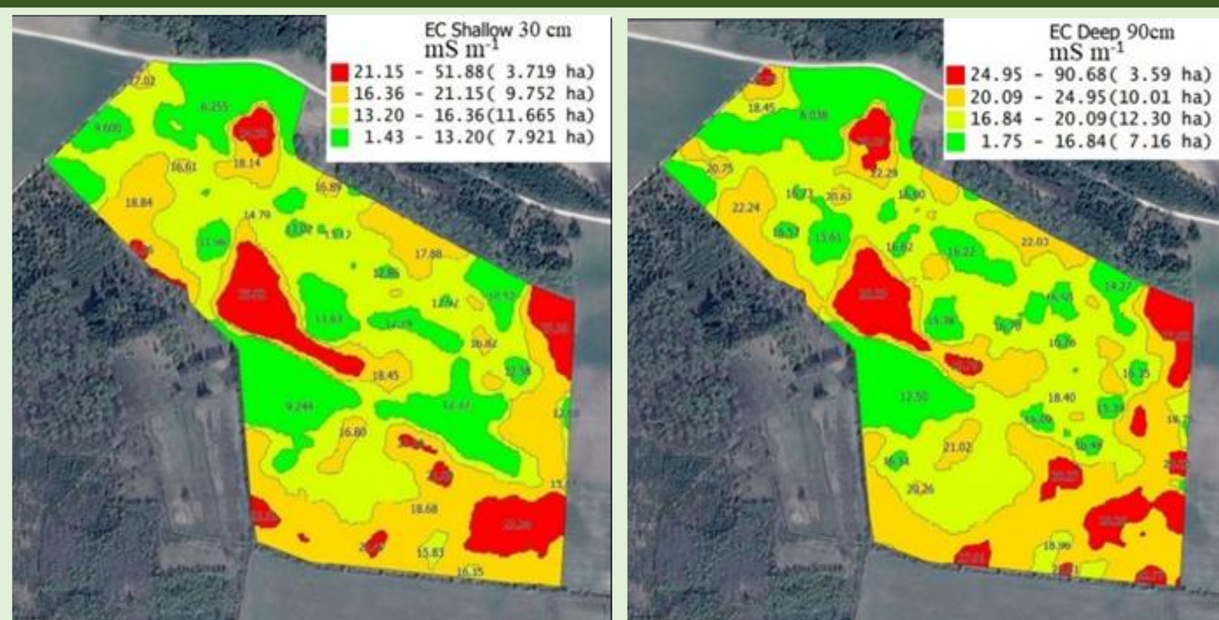
Figure 4. ECa maps of soil surface structure differences at the depth of 30 cm (left-hand-side) and 90 cm (right-hand-side) (colored parameter variation internal maps were created by the authors using Veris MSP 3150 and as a background layer was used ORT10LT - digital raster orthophoto map of the territory of the Republic of Lithuania M 1: 10000 (compiled 2012-2013) in the precision farming software AgLeader SMS Advanced).
