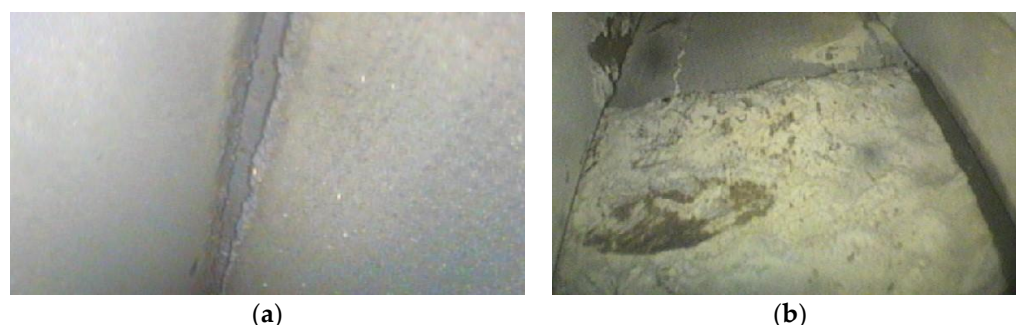
Figure 1. (a) Trace of PDs (2009), (b) Serious damage and traces of PDs inside the SG's stator (2010).
