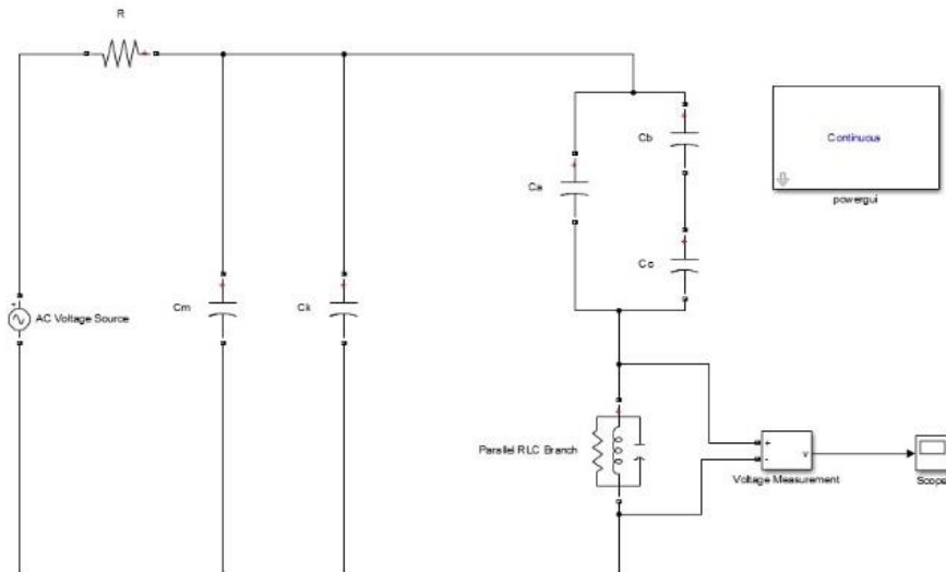
Figure 2. Capacitive Model.
