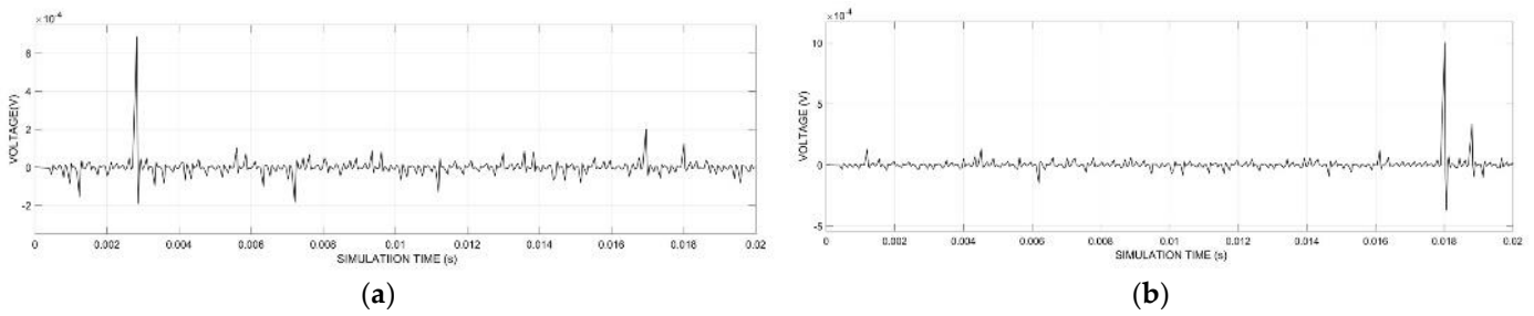
Figure 5. PD Activity—Combination (a) 15 kV, double height, (b) 15 kV—double radius.
