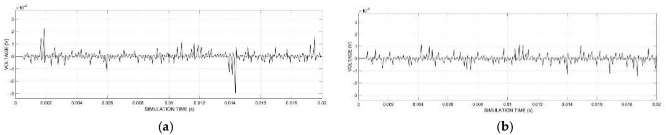
Figure 7. PD Activity—ER (a) 5 kV, (b) 5 kV—double radius.
