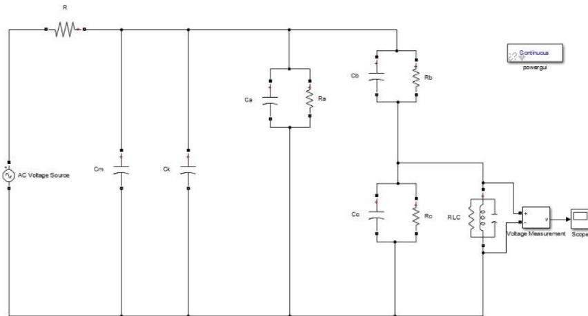
Figure 6. Capacitive-Resistance PD Model.
