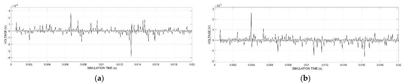
Figure 8. PD Activity—Mica (a) 10 kV, (b) 10 kV—double height.
