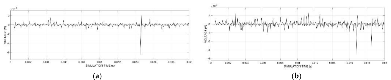
Figure 9. PD Activity—Combination (a) 15 kV, double height, (b) 15 kV—double radius.
