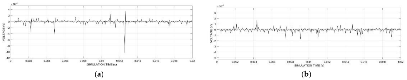
Figure 4. PD Activity—Mica (a) 10 kV, (b) 10 kV—double height.
