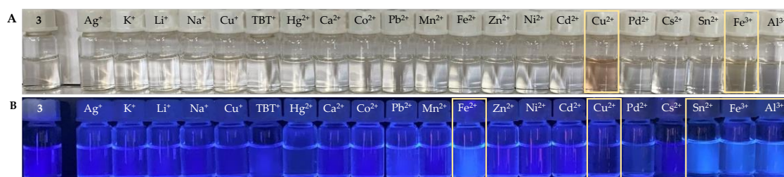
Figure 6. Solutions of compound 3 , in ACN/water (75:25) ( 1 \times 10^{-5} M), after adding 50 equivalents of cations, under natural light (A) and UV radiation at 365 nm (B).
