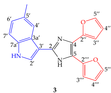
Figure 1. Structure of imidazole derivative 3 .
