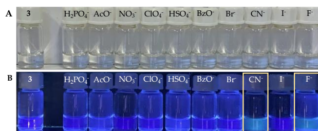
Figure 3. Solutions of compound 3 , in ACN ( 1 \times 10^{-5} M), after adding 50 equivalents of anions, under natural light (A) and UV radiation at 365 nm (B).
