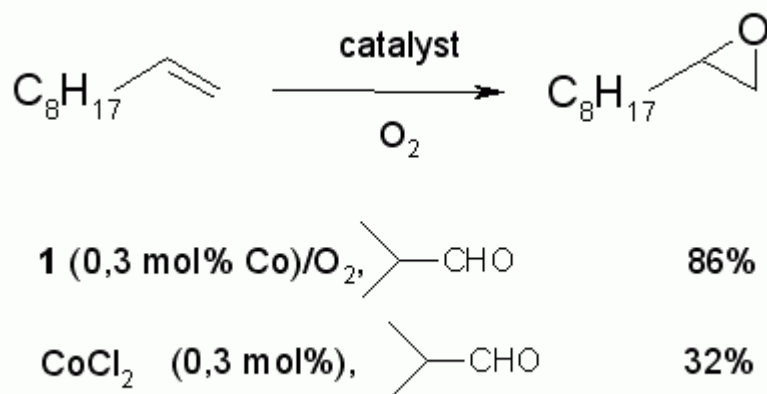
Scheme 2.
