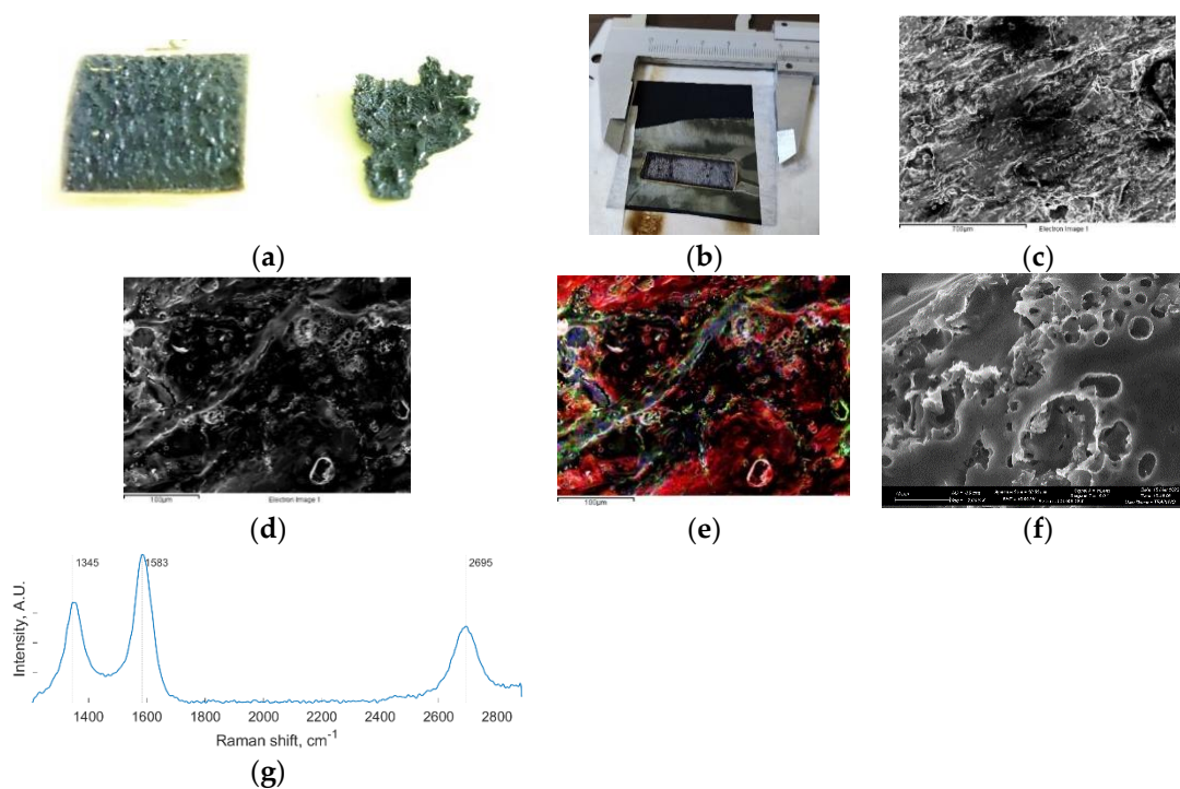
Figure 1. (a) Back side of the LIG-S with remaining SPEEK droplets; (b) LIG-S onto CP at the end of the laser scribing process; (c) Low magnification FESEM of the LIG-S surface; (d) Intermediate magnification FESEM of the LIG-S surface; (e) EDX map of (d) showing carbon (red), oxygen (green) and sulfur (blue); (f) High magnification FESEM of the LIG-S surface; (g) Raman spectrum of LIG-S: D peak \sim 1350\text{ cm}^{-1} , G peak \sim 1580\text{ cm}^{-1} , and 2D peak \sim 2700\text{ cm}^{-1} .
