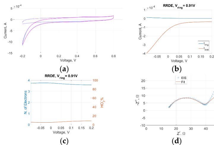
Figure 2. (a) CV at 10 mV/s scan rate in nitrogen and oxygen showing ORR activity. Both RRDE and GDE setups returned a curve with identical features. Here, only the GDE one is reported; (b) RRDE disk and ring current comparison; (c) Average detected number of electrons involved in the ORR
