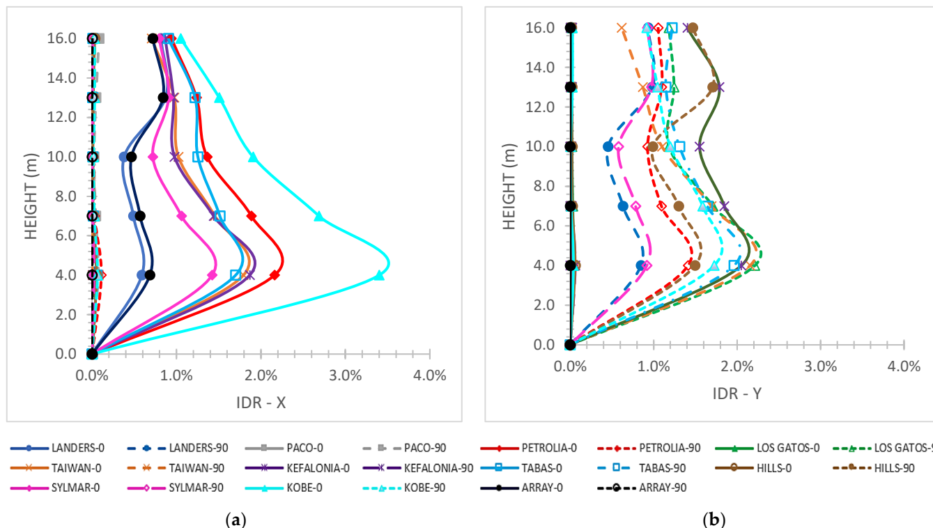
Figure 4. Interstory drift ratio on (X) and (Y) axes for the 5-story frame for the fixed-pinned support of the steel structure on the RC stories.
