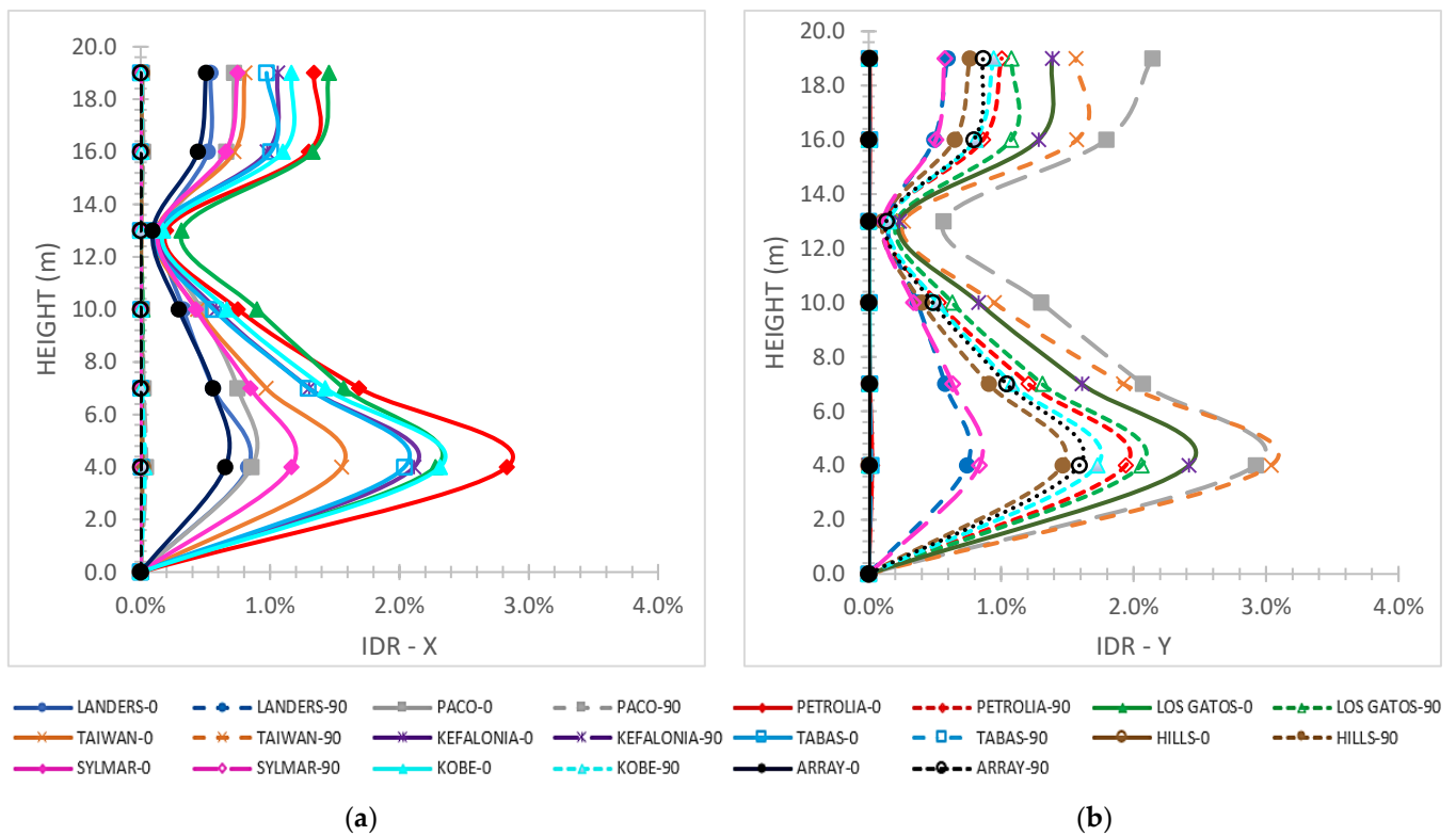
Figure 6. Interstory drift ratio on (X) and (Y) axes for the 6-story frame for the fixed-pinned support of the steel structure on the RC stories.
