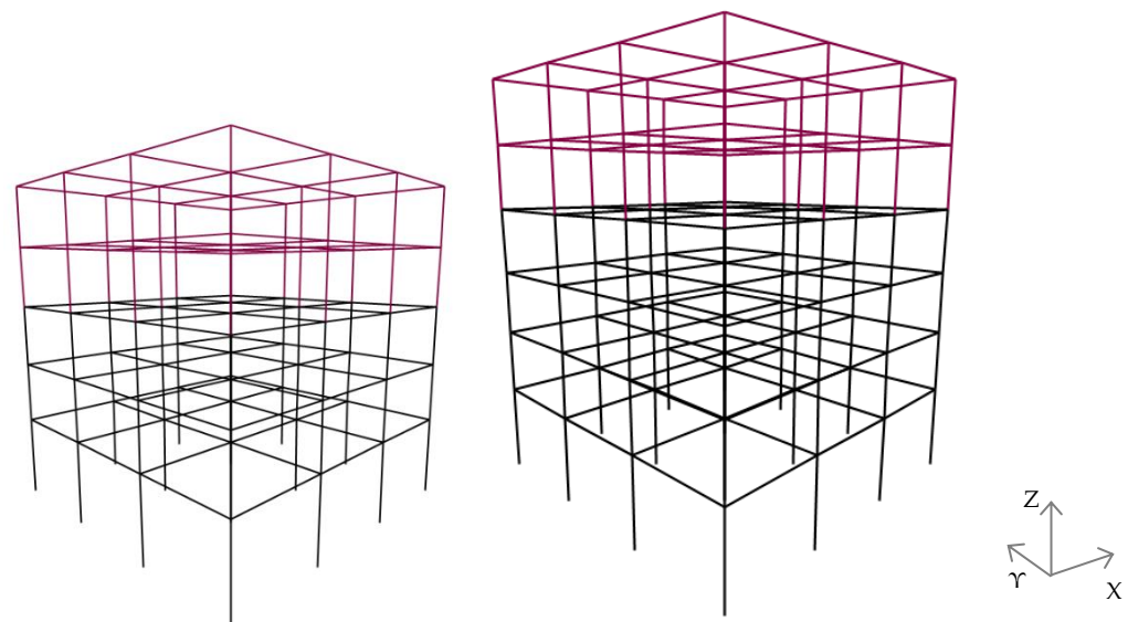
Figure 1. Five- and (c) six-story mixed RC-steel 3D frames under study (lower RC stories with black color and higher steel stories with crimson color) with a global coordinate system.
