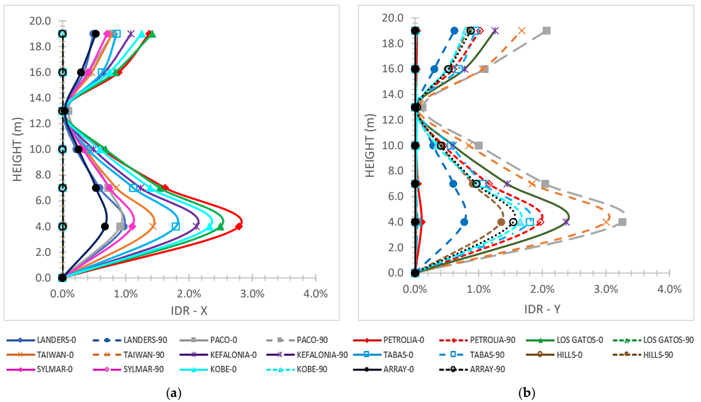
Figure 5. Interstory drift ratio on (X) and (Y) axes for the 6-story frame for the fixed support of the steel part on the RC one.
