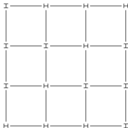
Figure 2. In-plan orientation of steel columns.
