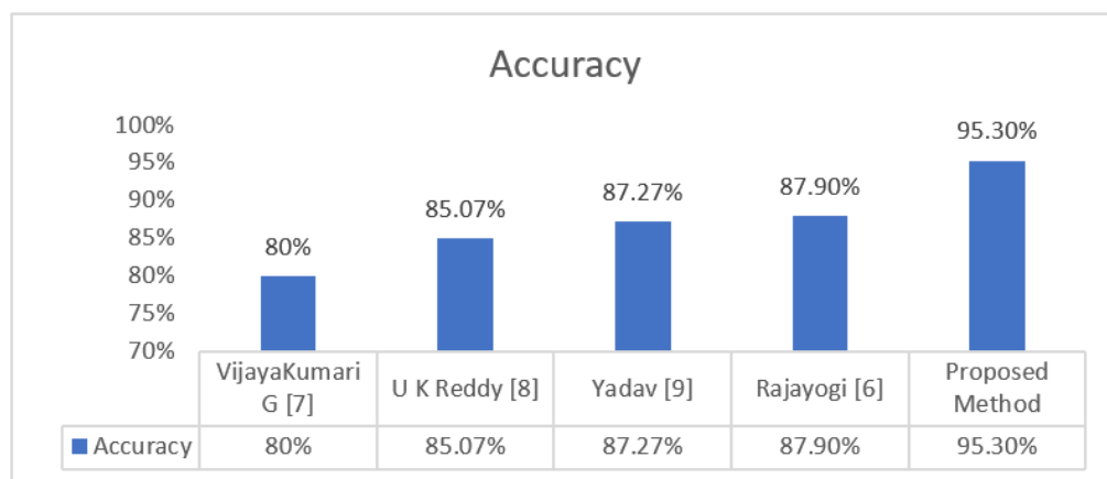
Figure 4. Result Comparisons with Past Related Work.
