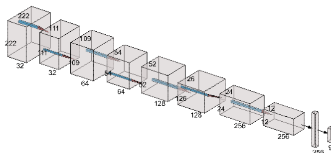
Figure 2. Architecture of Self-Designed CNN.
