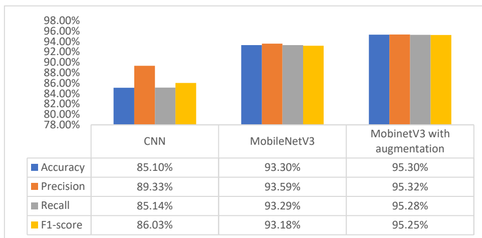
Figure 3. Result Comparisons of all models.
