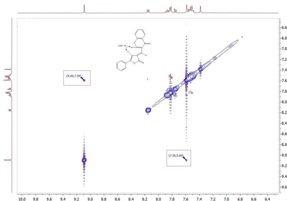
Figure 1. NOESY2D spectrum.
