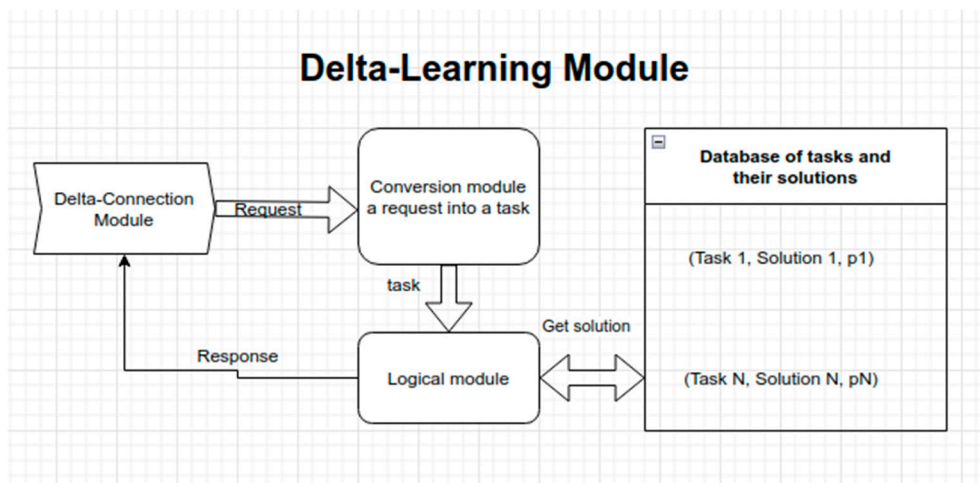
Figure 3. Delta-Learning Module.
