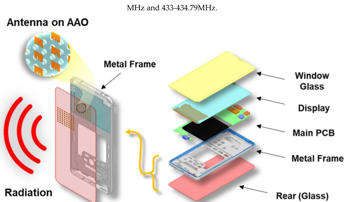
Figure 1. Materials used to make miniature antennas.
