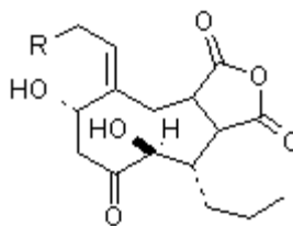
127 R = H cornexistine 128 R = OH hydroxycornexistine
