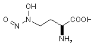
137 homoalanosine
