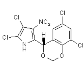
52 dioxapyrrolomycin
