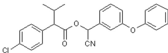
10 fenvalerate Sumitomo
