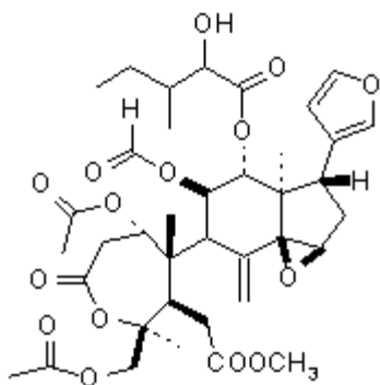
112 14,15[beta]-epoxy-prieurianin
