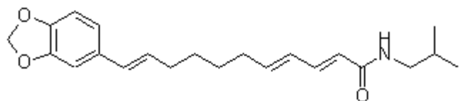
67 pipericide
