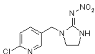
25 imidacloprid Bayer
