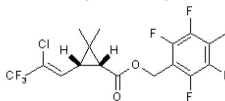
18 tefluthrin Zeneca
