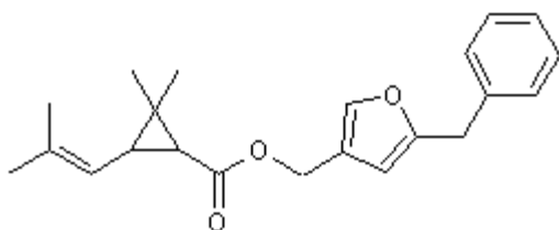
6 resmethrin Rothamstead
