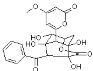
129 vulgamycin
