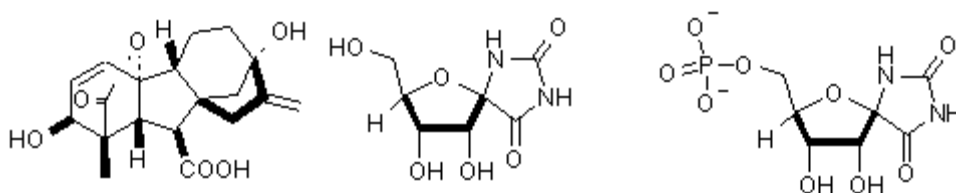
120 gibberellin A 3 121 hydantocidin 122 hydantocidin-5'-phosphate
