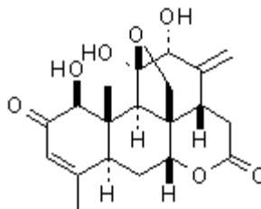
131 ailanthone
