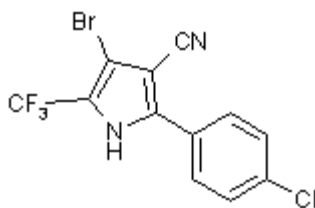
52 dioxapyrrolomycin
