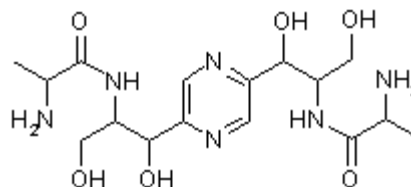
85 diabroticin A
