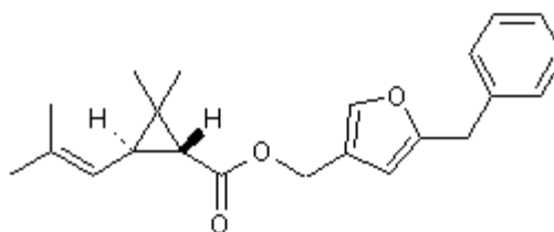
7 bioresmethrin Rothamstead
