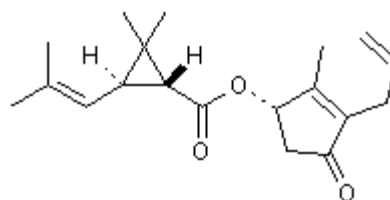
4 S -bioallethrin USDA, Roussel-Uclaf
