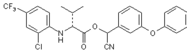
20 [tau]-fluvalinate Sandoz [1]
