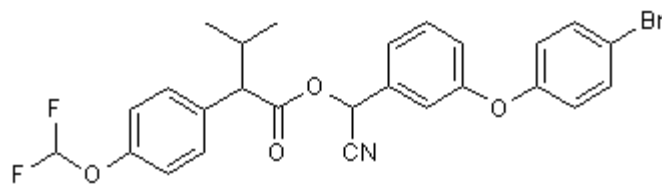
12 Zxi 8901 Shanghai Zhong-Xi
