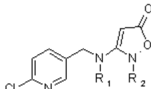
R 1 , R 2 = H, alkyl 29 lead structure Novartis
