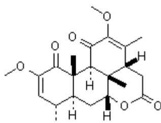
77 quassin
