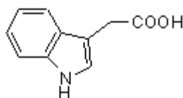
114 3-indolyl acetic acid
