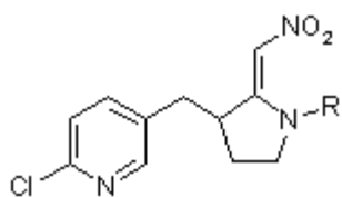
R = H, alkyl 28 lead structure Novartis
