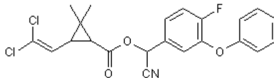
16 cyfluthrin Bayer
