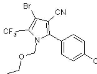
55 chlorfenapyr American Cyanamid
