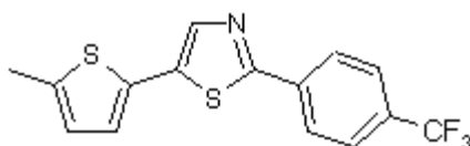
82 F-5183
