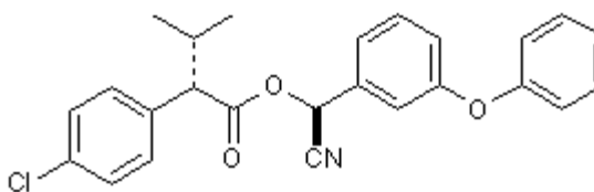
11 esfenvalerate Sumitomo
