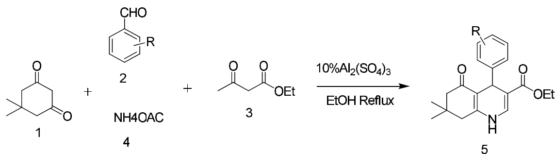
Figure 1 \text{Al}_2(\text{SO}_4)_3 catalyzed synthesis of Polyhydroquinoline derivatives
