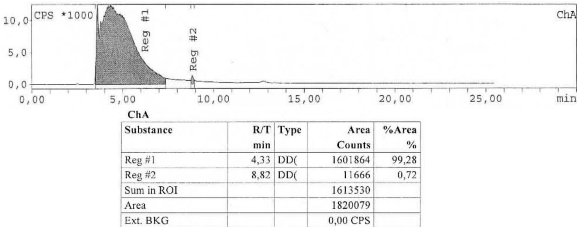
Figure 1. HPLC profile obtained for the complexation of the ^{99m}\text{Tc} and the tricarbonyl and its relative percentage, which informs about the radiochemical purity (RCP).
