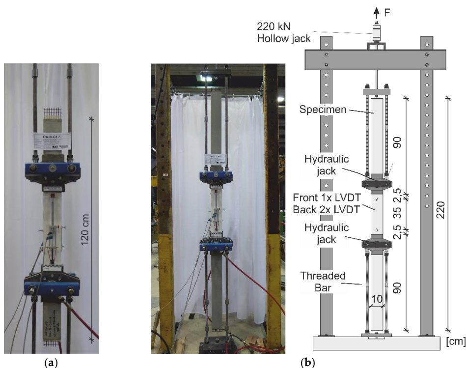
Figure 1. (a) Tensile test setup for specimen with additional coating with epoxy-resin and quartz sand in the anchorage zone; (b) Long tensile test setup for realistic anchorage conditions
