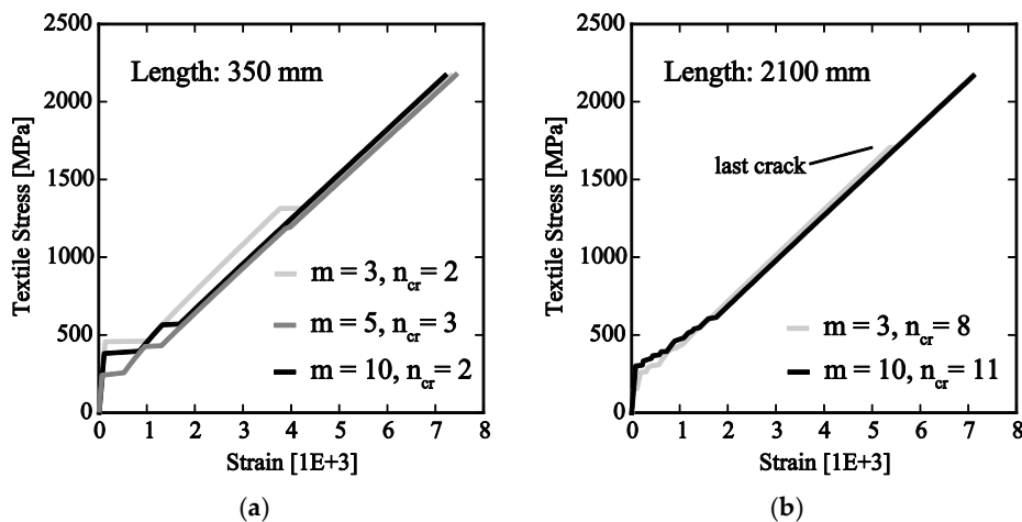
Figure 4. simulation of tensile test with random matrix strength (a) l=350 mm; (b) l=2100 mm
