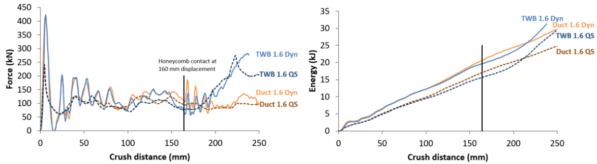
Figure 4: Comparison of crush response under dynamic (Dyn) and quasi-static (QS) conditions.
