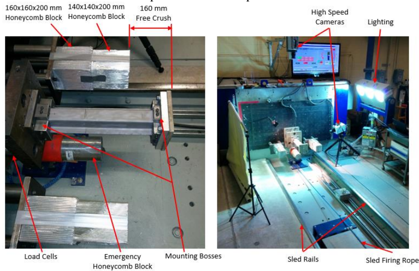
Figure 2: Dynamic axial crush test setup at UW. [6]
