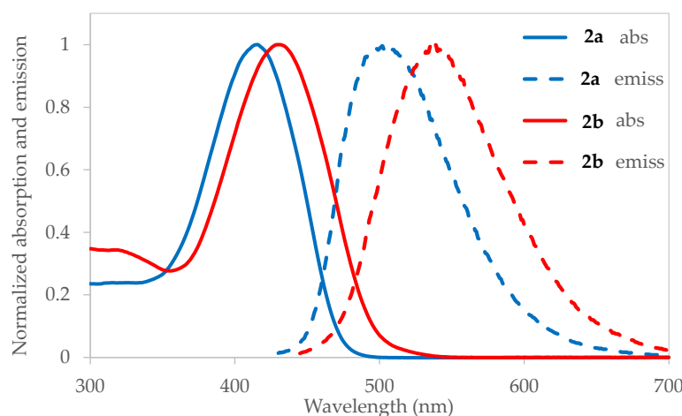
Figure 1. Normalized UV-vis absorption and emission spectra of compounds 2a and 2b in dioxane at T=298 K ( 2a , \lambda_{\text{exc}}=415 nm; 2b , \lambda_{\text{exc}}=430 nm) (absorption, full line; emission, dashed line).
