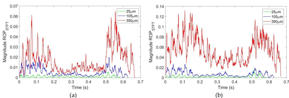
Figure 2. ROP of the (a) AE sensor and (b) PZT transducer.
