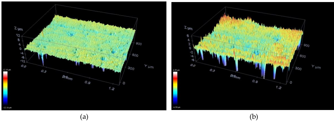
Figure 1. Confocal microscopy, (a) 25 μm and (b) 350 μm.
