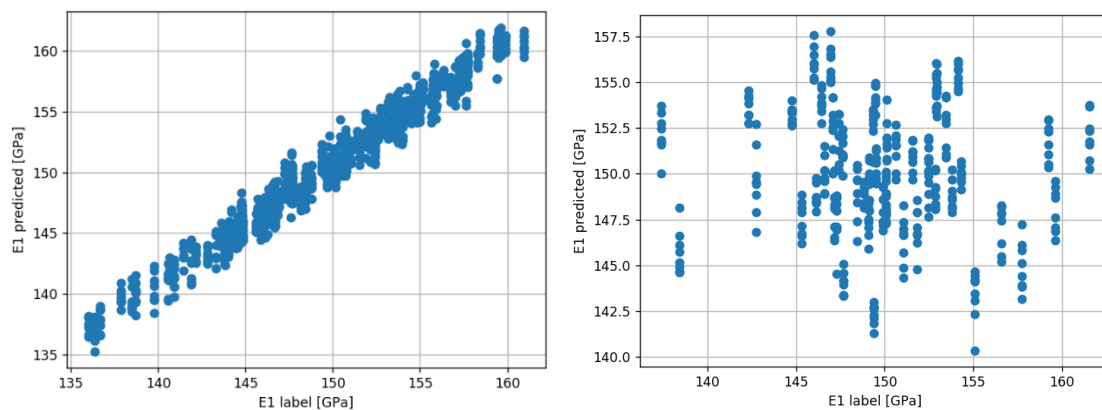
Figure 5. Effective Young’s modulus predicted by the NN against the ground-truth data: (left) training set; (right) validation set.
