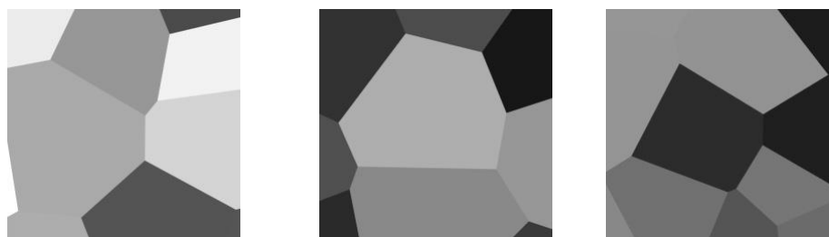
Figure 1. Exemplary morphologies of 2 \times 2 \mu\text{m}^2 SVEs, where each color represents a different grain.
