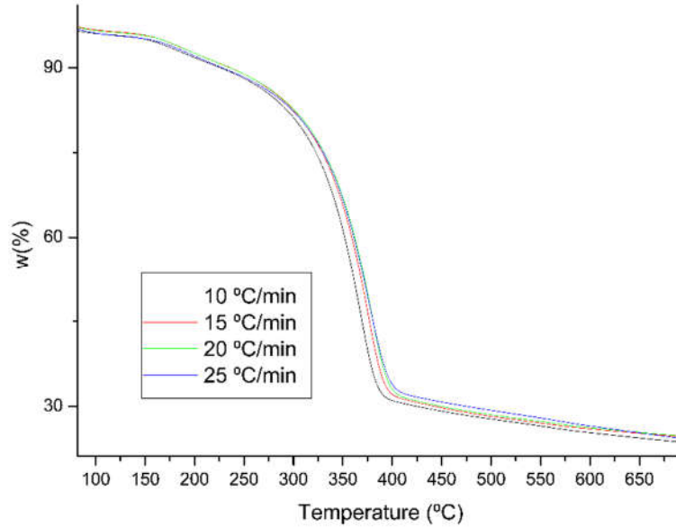
Figure 4. Experimental TG curves at different heating rates of chitin isolated from Vespa velutina .
