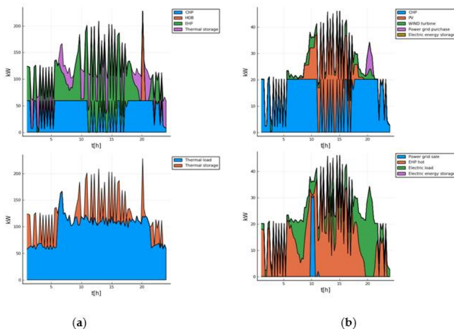
Figure 5. Daily consumption and production pattern for Case 1: (a) Thermal consumption; (b) Electricity consumption.
