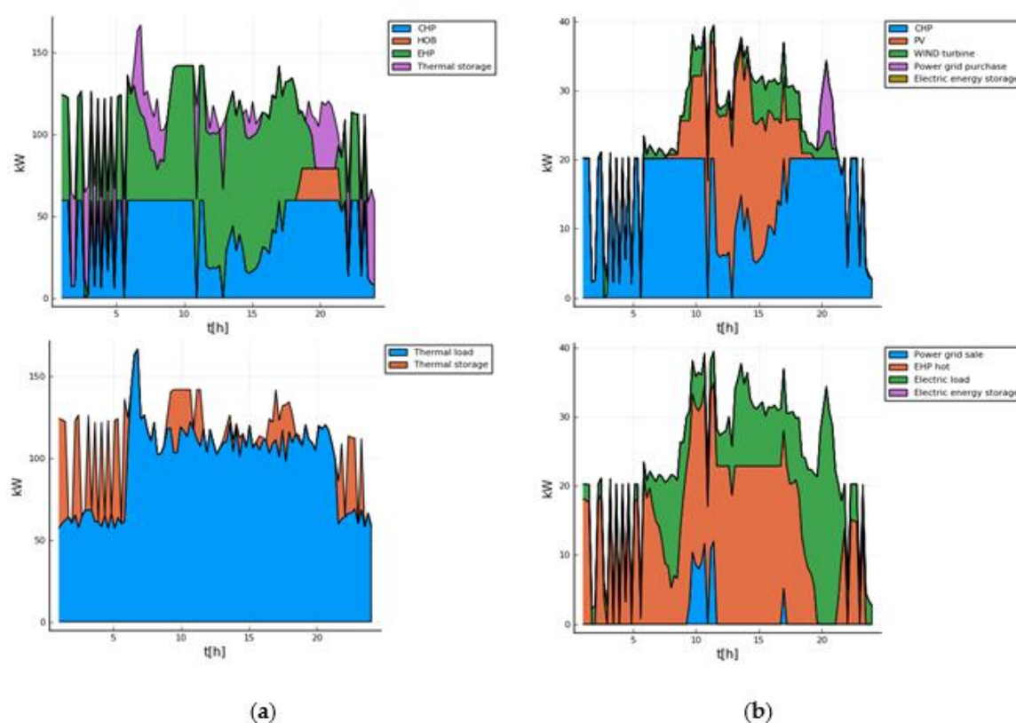
Figure 8. Daily consumption and production pattern in case of investment cost inclusion for the Case 1: (a) Thermal consumption; (b) Electricity consumption.
