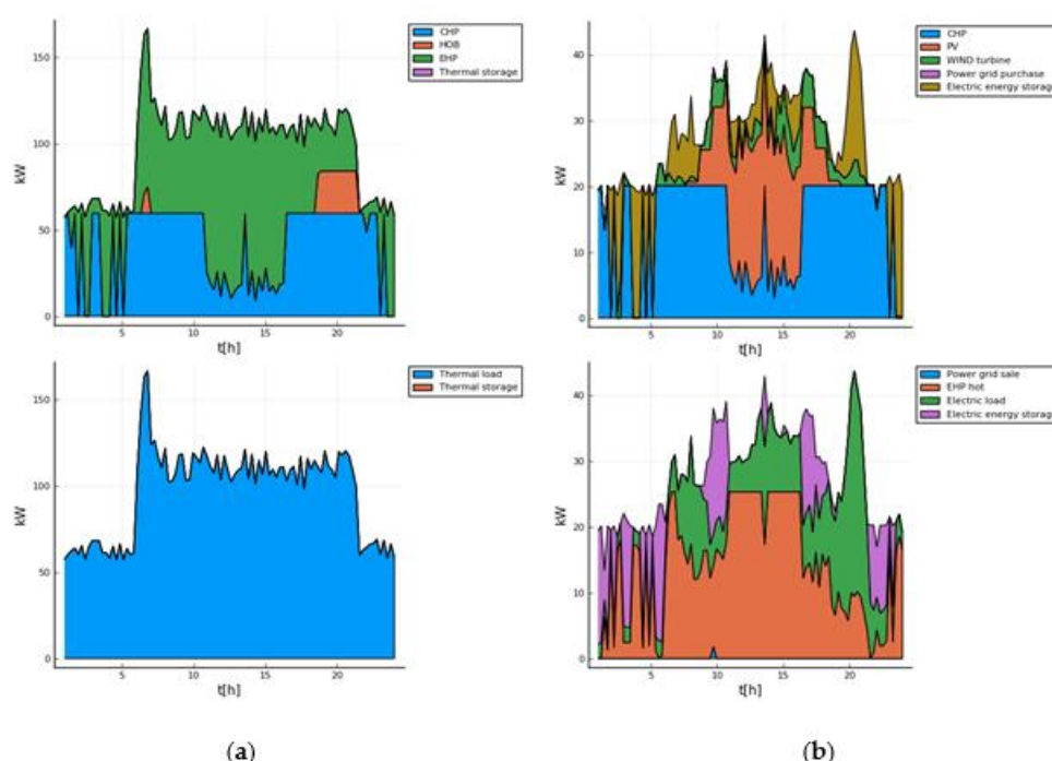
Figure 9. Daily consumption and production pattern in case of investment cost inclusion for the Case 2: (a) Thermal consumption; (b) Electricity consumption.
