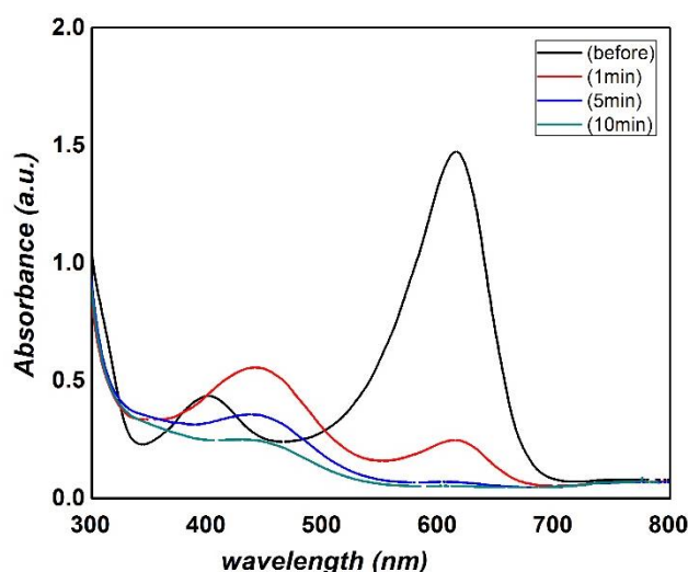
Figure 3. The recorded absorption spectra of solution samples for different duration plasma irradiation.
