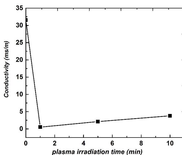
Figure 1. Variation of conductivity value of the sample solution after the different duration of plasma jet irradiation.
