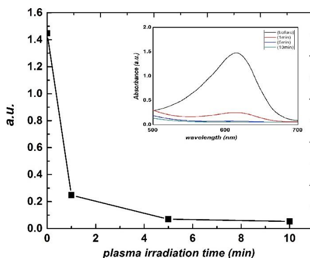
Figure 4. The decrease in the intensity of the absorption peak around 600 nm.
