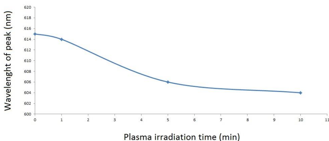
Figure 5. Change of the absorption peak wavelengths for different plasma jet irradiation durations.
