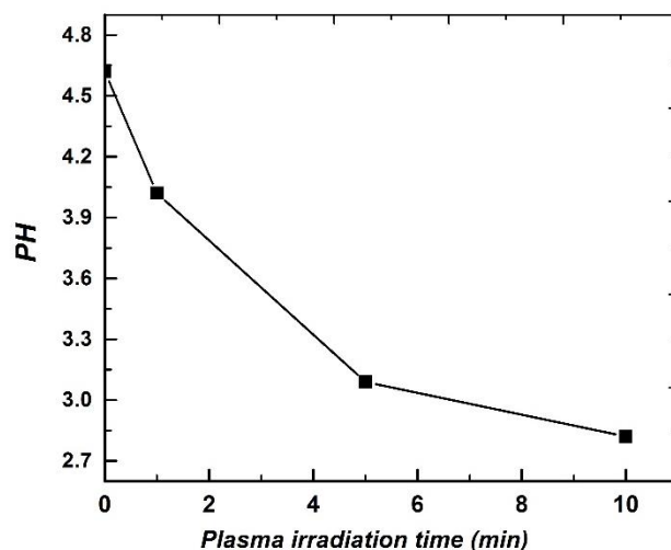
Figure 2. Variation of pH of the sample solutions with different durations plasma jet treatment.
