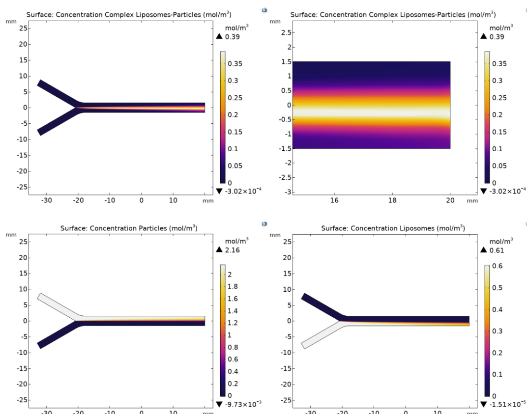
Figure 4. Concentration profiles of diluted species for K_{max} = 0.05 \text{ mM} and K_{cat} = 0.5 \text{ s}^{-1} ; (a) concentration of liposomes-particles complexes; (b) zoom at the outlet for the concentration of liposomes-particles; (c) concentration of particles; and (d) concentration of liposomes.
