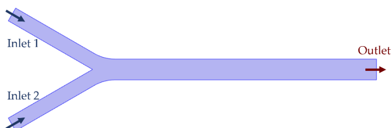
Figure 1. Computational domain and boundary conditions. Both 2.12 mm inlets converge in a 30° angle into a 3 mm width and 40 mm length channel.
