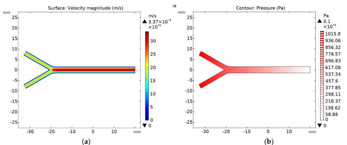
Figure 2. Hydrodynamics of ferrofluid in a laminar flow regime within the microfluidic device: (a) Velocity field profile results; (b) pressure field contour results.
