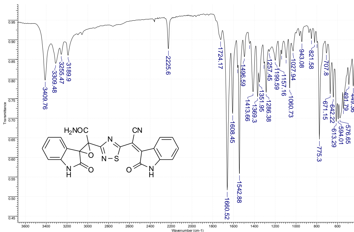
Figure 1. FT-IR (ATR mode) spectrum of compound 6.
