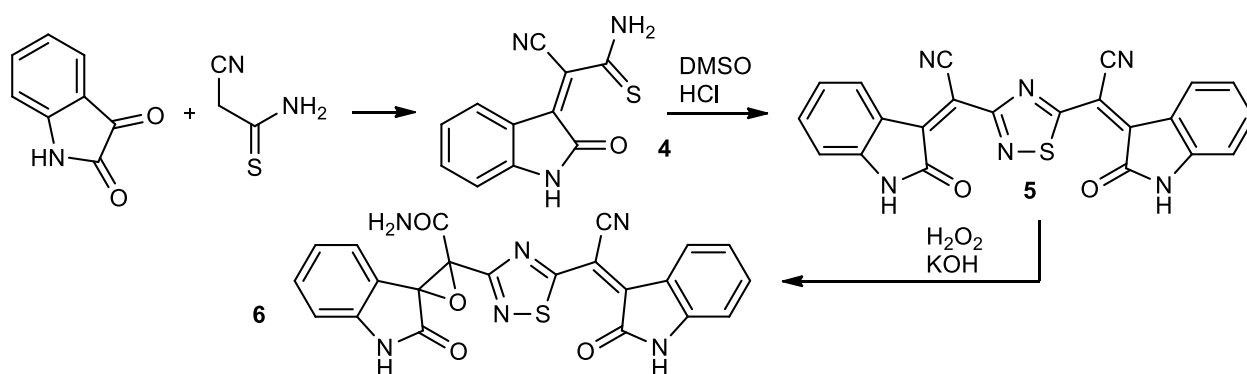
Scheme 2. Synthesis and oxidation of thioamides 4 .
