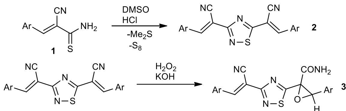
Scheme 2. Synthesis and oxidation of 3,5-di( \alpha -cyanostiryl)-1,2,4-thiadiazoles 2 .
