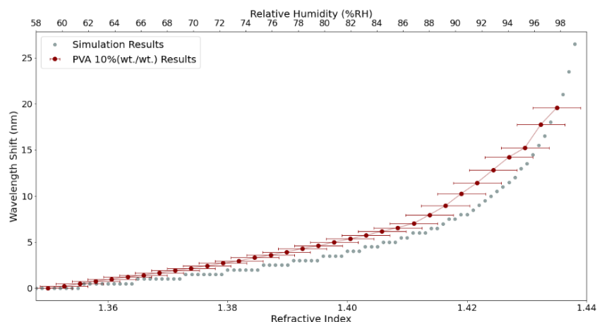
Figure 3. Comparison between the wavelength shift of experimental 10%wt/wt PVA LPFG and the simulations of as function the external refractive index.
