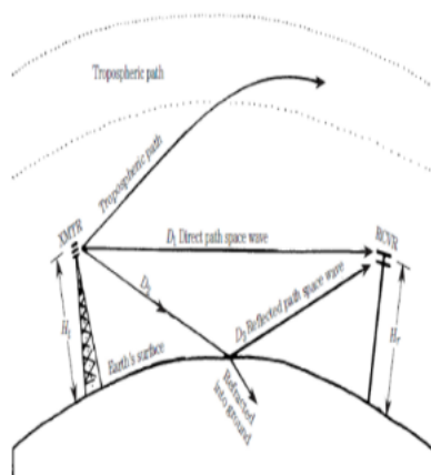
Fig. 1 Showing Space Wave Propagation [3]
