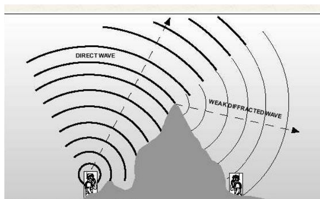
Fig. 5: Showing VHF and UHF Diffraction. [2]
