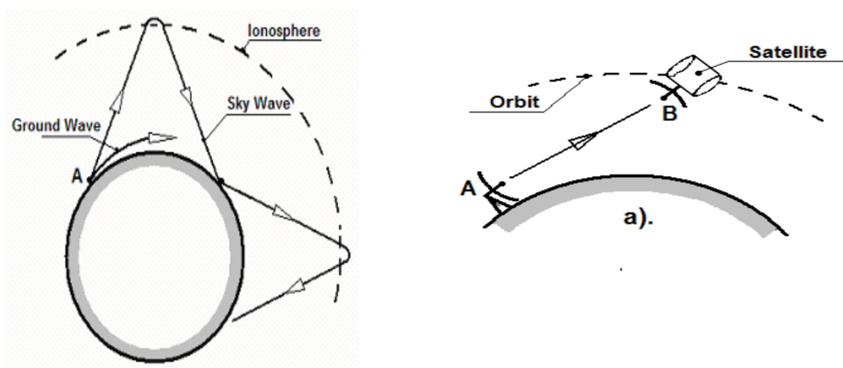
Fig.2 Showing Sky Wave Propagation [1]
