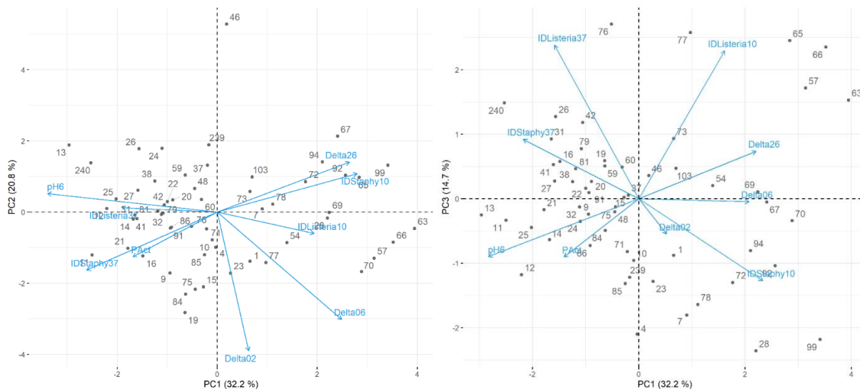
Figure 1. Maps of the first and second principal components (left) and the first and third principal components (right) of the tested technological properties of MRS-isolated LAB.
