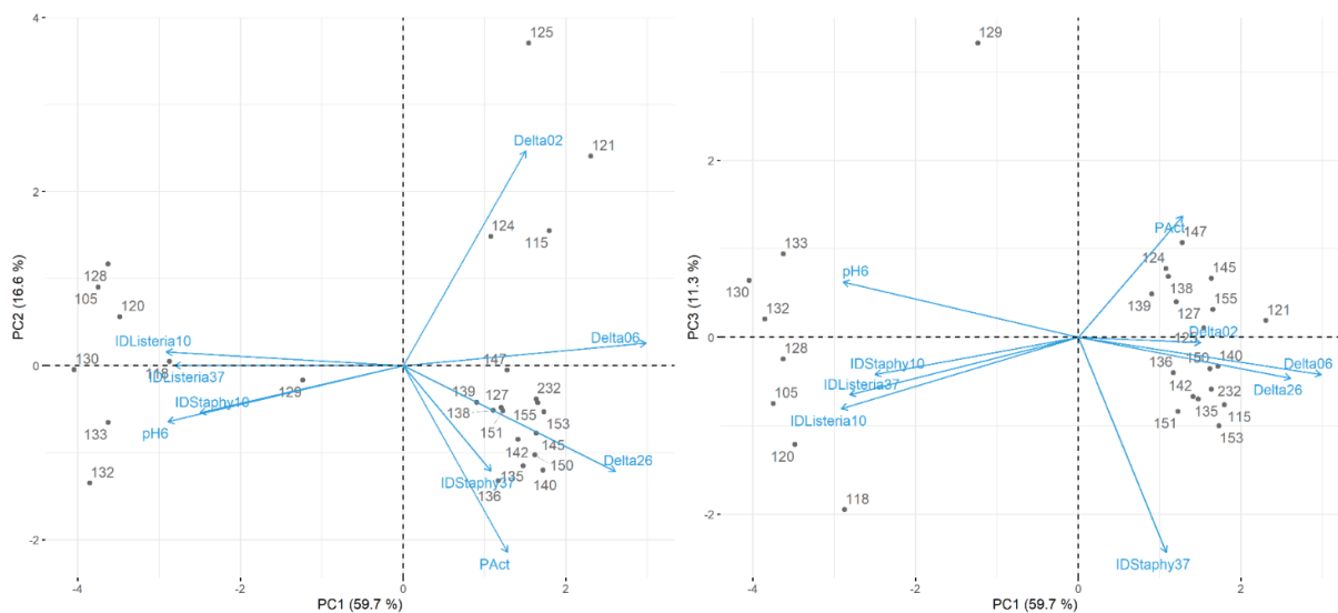
Figure 2. Maps of the first and second principal components (left) and the first and third principal components (right) of the tested technological properties of M17-isolated LAB.
