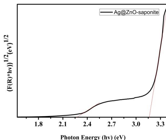
Figure 2. Band gap value ( E_g ) of Ag@ZnO-saponite determined according to the Kubelka–Munk method by using the Tauc equation.
