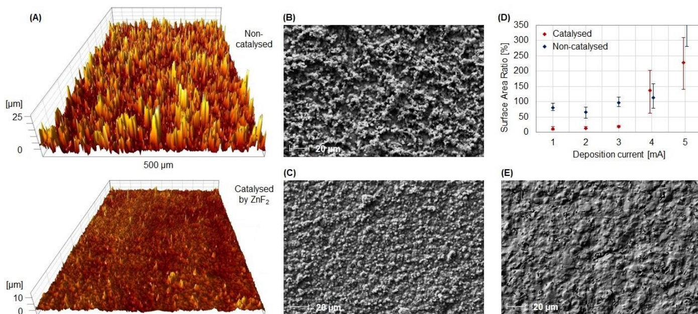
Figure 2. Surface topography of electropolymerized polythiophene films. (A) 3D white light images of films deposited with 3 mA with and without the catalyst ZnF_2 . (B,C) Complementary SEM images of the same films. (D) Surface area ratio of films deposited with currents ranging from 1–5 mA. (E) SEM image of a clean, uncoated electrode.
