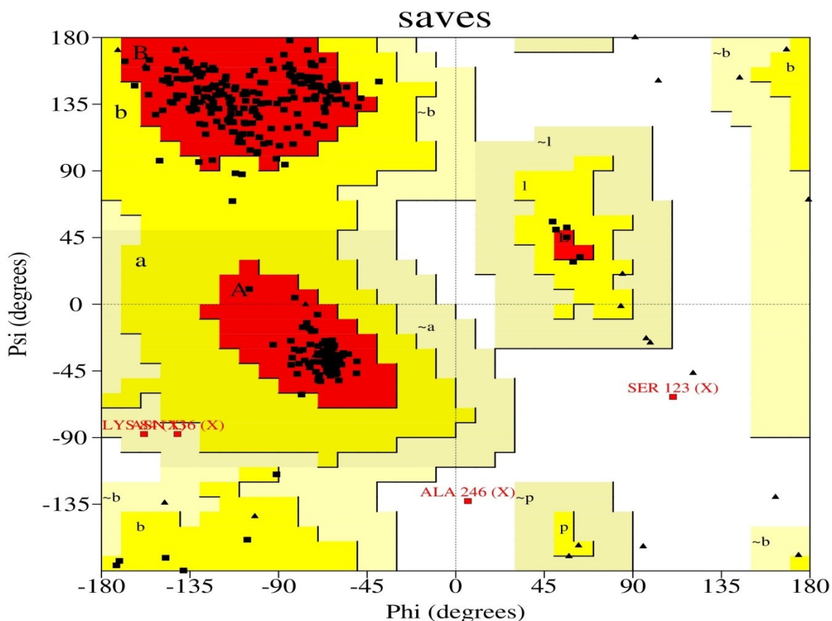
Figure 3. The Ramachandran plot statistics of Modeller-predicted three-dimensional protein structure validated by the PROCHECK program.
