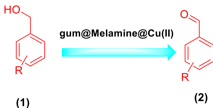
Scheme 1. Synthesized derivatives in oxidation reaction.
