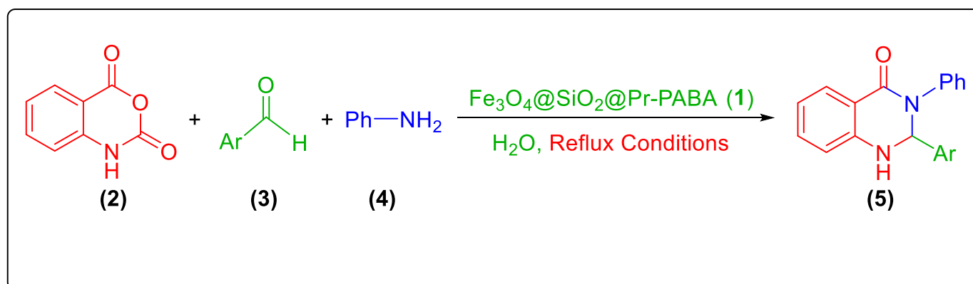
Scheme 1. Synthesis of 2,3-dihydroquinazolin-4(1H)-one derivatives catalyzed by \text{Fe}_3\text{O}_4@\text{SiO}_2@\text{Pr-PABA} (1).
