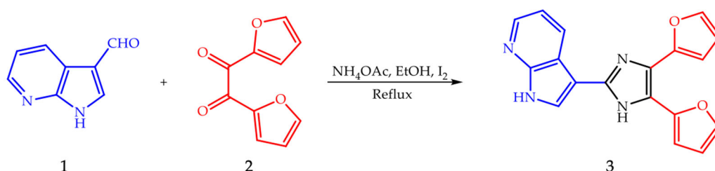
Scheme 1. Synthesis of imidazole derivative 3 .
