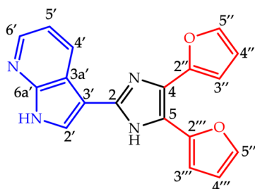
Figure 1. Structure of imidazole derivative 3 .
