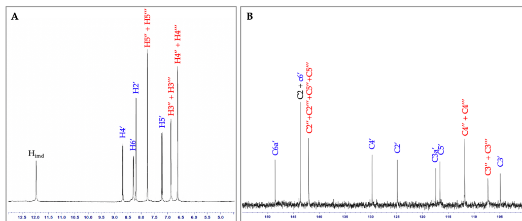
Figure 2. ^1\text{H} NMR (A) and ^{13}\text{C} NMR (B) spectra of imidazole derivative 3.
