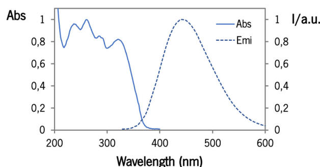
Figure 3. Normalized absorption and emission spectra of imidazole derivative 3.
