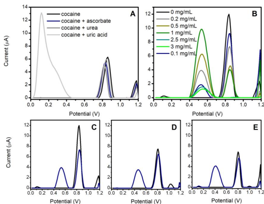
Figure 3. Investigation of the OF matrix effects on 10 \mu\text{M} cocaine under optimal conditions: (A) Effect of OF constituents: ascorbate, urea, uric acid and (B) effect of albumin concentration. Effect of the pH on the oxidation signal for 10 \mu\text{M} cocaine in the presence of 0.2 \text{mg mL}^{-1} albumin with (C) pH 9, (D) pH 10, and (E) pH 11. Black line: 10 \mu\text{M} cocaine, blue line: 10 \mu\text{M} cocaine in the presence of 0.2 \text{mg mL}^{-1} albumin. All tests were executed in BR buffer containing 0.075 \text{mg mL}^{-1} SDS.
