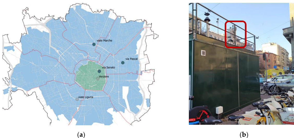
Figure S1. Assessment of near reference sensors stations. (a) Monitors' geographical location, represented as blue dots either within the 'Area C' Congestions Charge Zone (green area) or the 'Area B' Low Emission Zone (blue area); (b) Collocation of the near reference monitor (within the red rectangle), with the via Senato reference monitor station.
