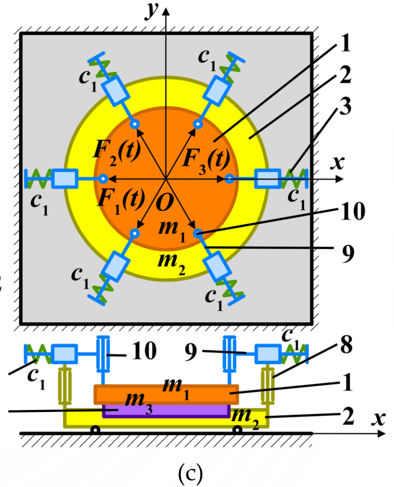
Figure 1. Vibratory lapping machine: (a) 3D-design; (b) electromagnets connection scheme; (c) kinematic diagram.
