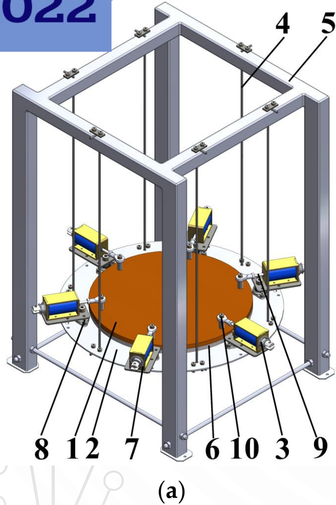
Figure 1. Vibratory lapping machine: (a) 3D-design; (b) electromagnets connection scheme; (c) kinematic diagram.
