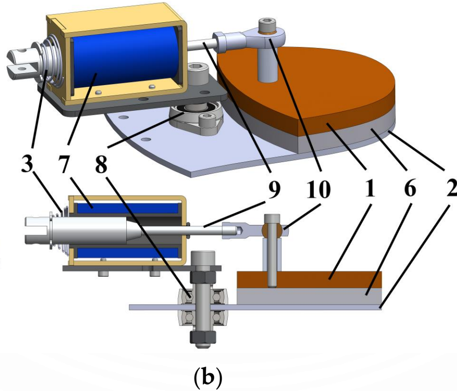
Figure 1. Vibratory lapping machine: (a) 3D-design; (b) electromagnets connection scheme; (c) kinematic diagram.
