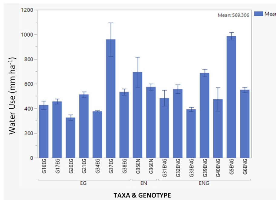
Figure 3. Average annual water use ( mm\ ha^{-1} ) for each selected genotype evaluated across all evaluated sites from 2017 to 2018.
