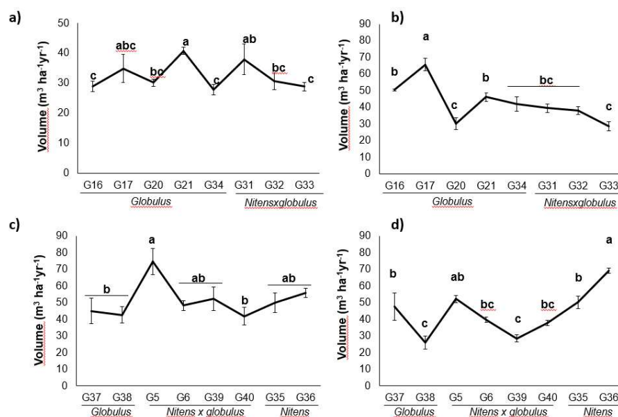
Figure 2. Average volume growth ( m^3\ ha^{-1}\ yr^{-1} ) of each genotype by taxa at a) Los Patos and b) Vegas de Saldia North sites, and c) El Derrumbe and d) San Andrés sites from 2017 to 2018.
