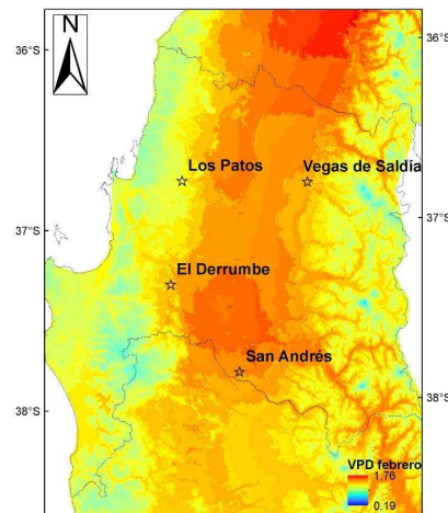
Figure 1. Mean daily vapour pressure deficit during February summer month map representing the regional gradient in atmospheric water demand for all sites selected and genotypes within each site.
