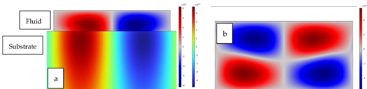
Figure 3. Standing pressure wave distribution in the microchannel (a) 50 \mu\text{m} , and (b) 140 \mu\text{m} thick.
