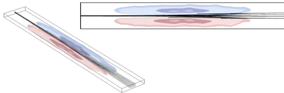
Figure 5. Particle trajectories, with the focusing effect achieved due to the ARF and the drag force.
