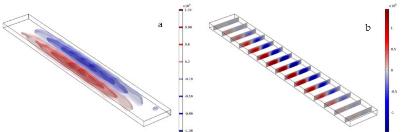
Figure 4. Acoustic pressure distribution within the fluid domain.
