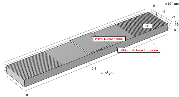
Figure 1. Geometry of the SAW-base device. The tags indicate the position of each component.
