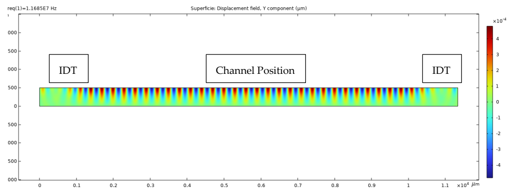
Figure 2. Numerical results in terms of vertical displacement, showing the formation of a standing surface wave. The tags indicate where the components of the device are placed.
