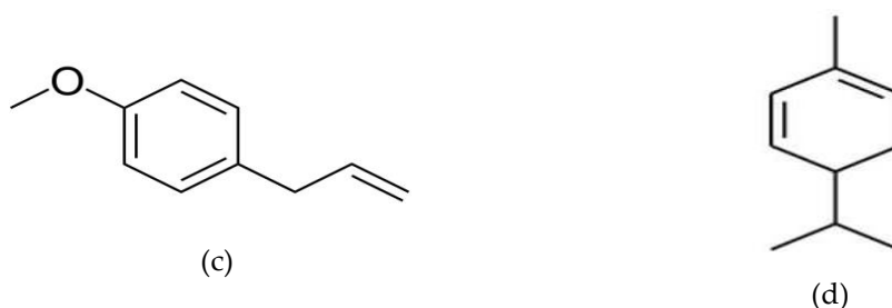
Figure 3. The molecule structures of the major bioactive essential oil component of F.vulgare . (a) Trans-anethole; (b) Fenchone; (c) p-anisaldehyde; (d) alpha-phellandrene.
