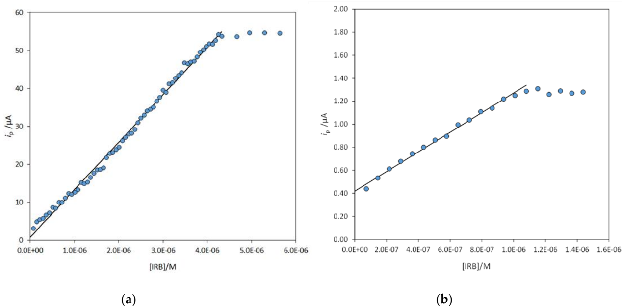
Figure 4. (a) Calibration curve of a non-functionalized electrode. (b) calibration curve of a MIP-functionalized electrode.
