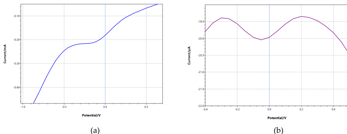
Figure 3. a) Square Wave Voltammogram of Irbesartan reduction on a bare electrode ([IRB] = 0.2 nM). b) Square Wave voltammogram of irbesartan reduction on a MIP-functionalized electrode ([IRB] = 0.2 nM).
