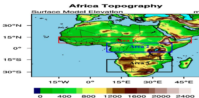
Figure 1. The figure shows the model domain and topography elevation (unit: meters).
