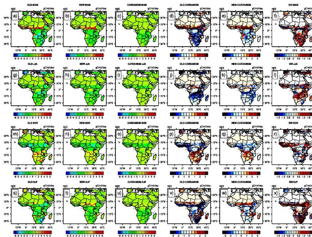
Figure 4. The figure shows the Net Ecosystem Exchange (NEE) over the period 2001–2010 (in gC\ m^{-2}\ day^{-1} ) for: MAM season in the first row (a-f); JJA in the second (g-l); SON in the third (m-r), DJF in the fourth (s-x). For each row, LAIorg (OLD) is on the left, followed by LAIorg (NEW), CARDAMOM is in the third from left, OLD minus CARDAMOM, NEW minus CARDAMOM and the difference between NEW and OLD. Significant model bias is indicated in black dots using student t-test with \alpha=0.05 .
