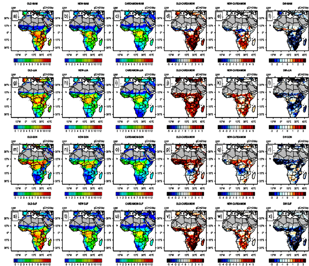
Figure 3. The figure shows the Gross Primary Production (GPP) over the period 2001–2010 (in gC\ m^{-2}\ day^{-1} ) for: MAM season in the first row (a-f); JJA in the second (g-l); SON in the third (m-r), DJF in the fourth (s-x). For each row, LAorg (OLD) is on the left, followed by LAmod (NEW), CARDAMOM is in the third from left, OLD minus CARDAMOM, NEW minus CARDAMOM and the difference between NEW and OLD. Significant model bias is indicated in black dots using student t-test with \alpha=0.05 .
