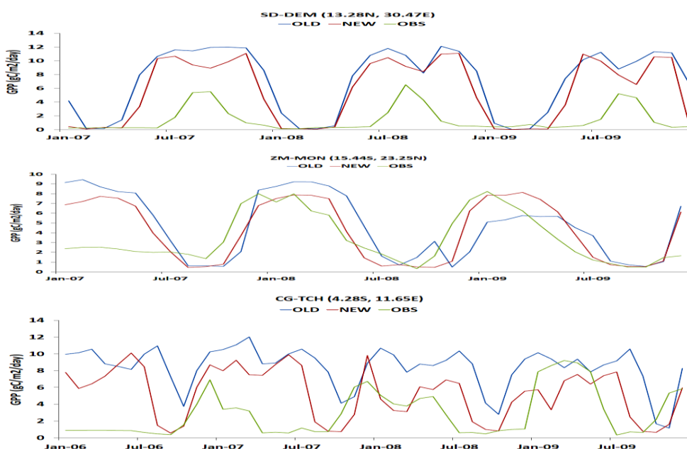
Figure 5. The figure shows the monthly mean GPP (in gC\ m^{-2}\ day^{-1} ) for the LAIorg (OLD; in blue), LAIorg (NEW; in red) and Fluxnet observation (in green) for the locations: SD-DEM (first row), ZM-MON (second row) and CG-TCH (third row).
