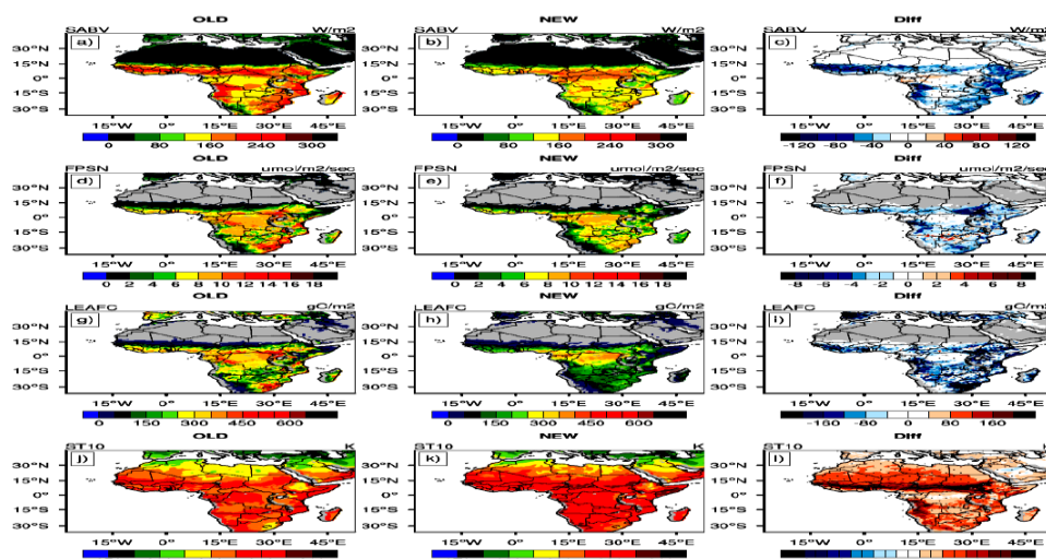
Figure 2. The figure shows the spatial pattern of the solar radiation absorbed by the vegetation (SABV; in \text{W m}^{-2} ; a-c), photosynthesis rate (FPSN; in \mu\text{mol m}^{-2} \text{sec}^{-1} ; d-f), leaf carbon (LEAFC; in \text{gC m}^{-2} ; g-i) and soil temperature of depth 10 cm (ST10; in K; j-l) over the period 2001 - 2010 for the simulations LAIorg (OLD), LAImod (NEW) and the significant difference (Diff) between the two simulations. The significant difference was calculated using student t-test with \alpha=0.05 .
