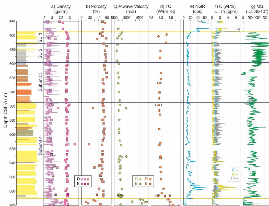
Figure 3. Petrophysical properties data acquired from the core sections and discrete samples at Hole D (440–700 m CSF-A) and Hole E (685–688 m CSF-A). The section of volcanoclastic-rich sequence (Unit V) is indicated by unit boundaries, subunits 1–4, and lithologic profile [3]. (a) Bulk density ( \text{g}/\text{cm}^3 ; purple line and square) and grain density ( \text{g}/\text{cm}^3 ; pink square). Purple line shows bulk density measured using GRA. (b) Porosity (%). (c) P -wave velocity (m/s). (d) Thermal conductivity (TC; \text{W}/(\text{m}\cdot\text{K}) ). Averaged values are shown (orange dot). (e) NGR spectral data (counts per second; cps) and (f) estimated abundance of K (wt.%), Th (ppm), and U (ppm). (g) Magnetic susceptibility (MS) data. Instrument unit (IU) was converted to dimensionless Système International (SI) unit [16].
