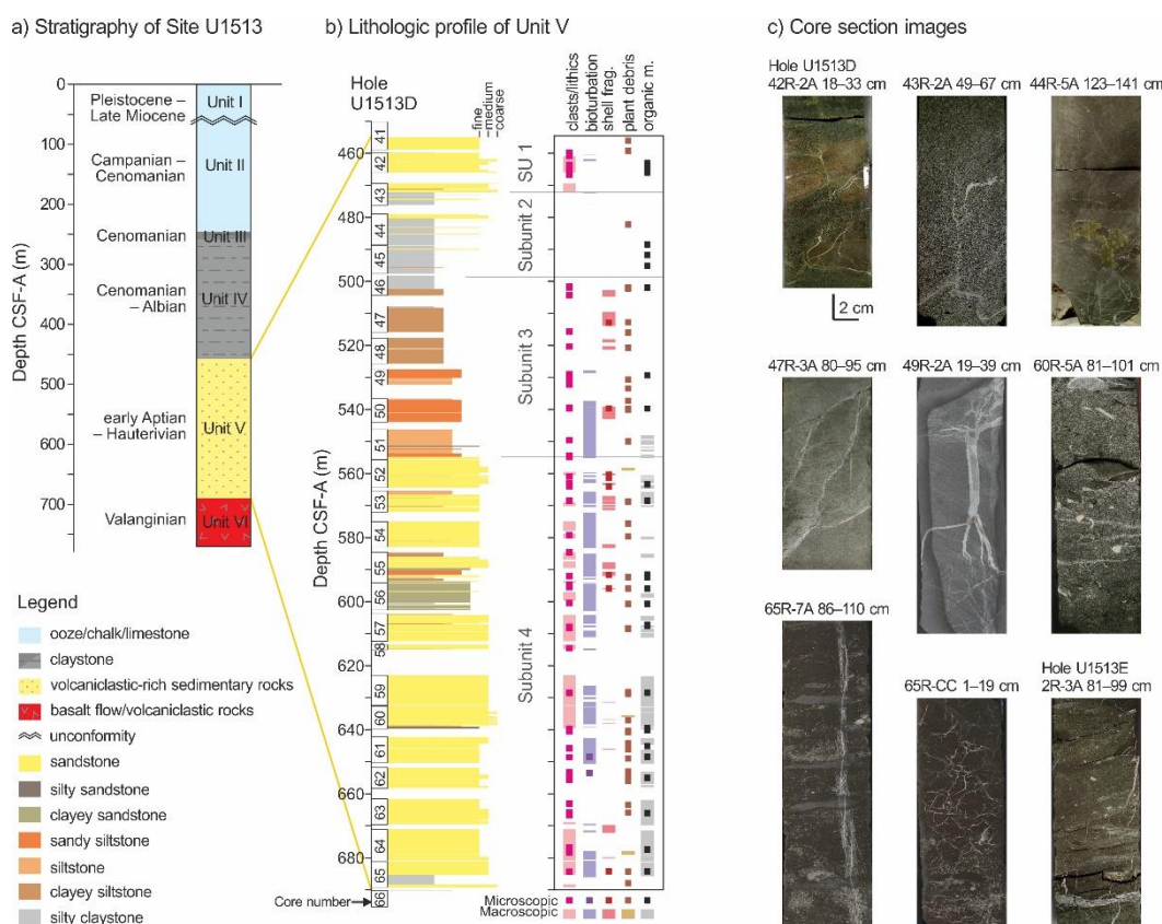
Figure 2. (a) Stratigraphy of IODP Site U1513 with Lithostratigraphic Units I to VI and geologic age [5]. (b) Lithologic profile of the volcaniclastic-rich sedimentary sequence (Unit V) at Hole U1513D with Subunits 1–4, core numbers, and macroscopic and microscopic observations. Distributions of volcanic clasts, lithic fragments, bioturbation, shell fragments, plant debris and unidentified organic matter are shown [3]. (c) Section images of Unit V showing distinct features including hydrothermal veins, calcite cementation, pyrite nodules, bioturbation, shell fragments, and fractures, and shell fragments. Section information (core-section, interval) of each image is shown.
