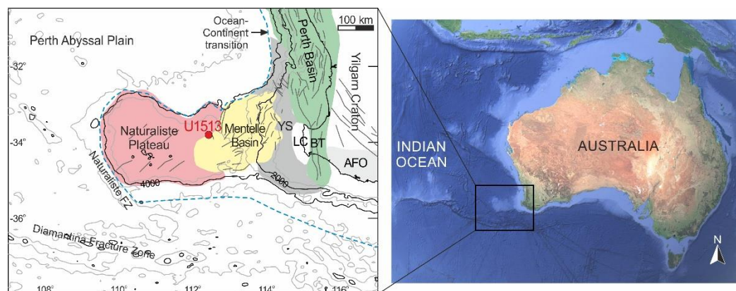
Figure 1. Structural setting of the southwestern Australian rifted margin and adjacent regions in the southeast Indian Ocean; Naturaliste Plateau, Mentelle Basin, Perth Abyssal Plain, Perth Basin, Yilgarn Craton, Yallingup Shelf (YS), Leeuwin Complex (LC), Bunbury Trough (BT), Albany-Fraser Orogen (AFO). Location of IODP Site U1513 on the eastern flank of the Naturaliste Plateau is shown. Thin gray lines show bathymetry (contour interval = 1,000 m). Blue dashed line indicates the ocean-continent transition (revised from [4]).
