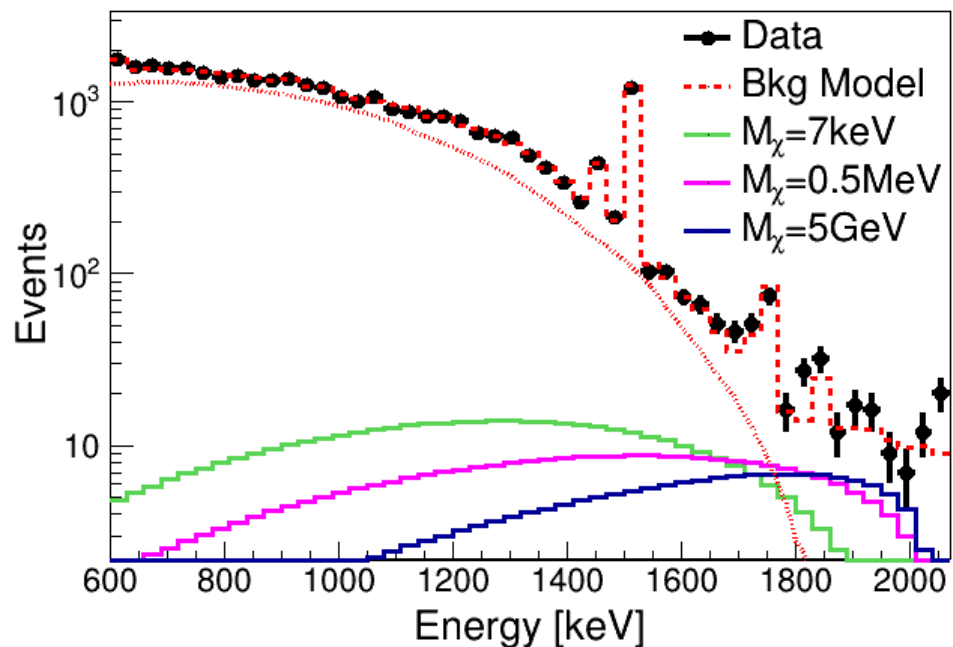
Figure 2. Upper limits on Dark Matter signals allowed by the "golden data-set" 17.9 kg x day exposure collected by Gerda Phase-I (points). The maximum signal allowed at 90% C.L. is shown for M_\chi=7\text{keV} , 0.5\text{MeV} and 5\text{GeV} (green, magenta and blue lines) respectively.
