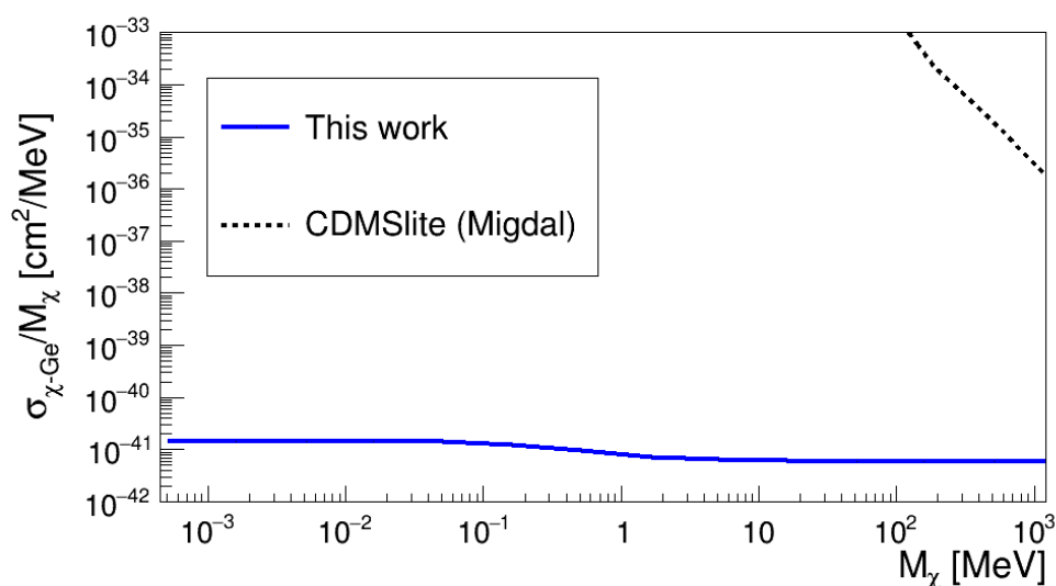
Figure 4. Example of upper limits on the total Dark Matter - Germanium nucleus cross section, obtained in this work considering the 17.9 kg x day exposure collected by Gerda Phase-I golden data set (blue line). Dotted line shows, as a comparison, the upper limits for the Dark Matter-Germanium nucleus elastic scattering for the very low mass region accessible exploiting the "Migdal effect" [17,18].
