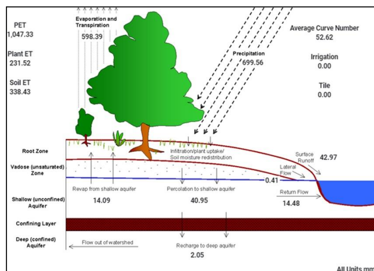
Figure 2. Schematic representation of water balance average annual values. All units in mm.
