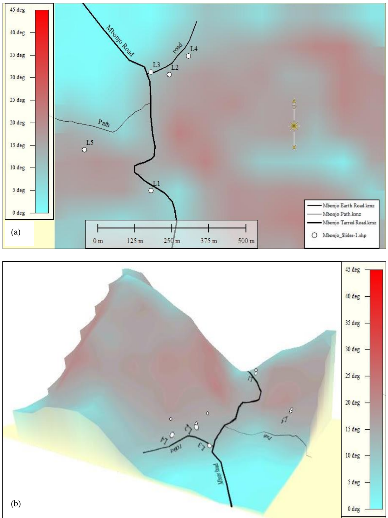
Figure 6. (a) SRTM slope shader showing gradients at which most of the studied landslides occurred; (b) 3D slope gradient map highlighting the occurrence of the studied landslides on steep slopes.
