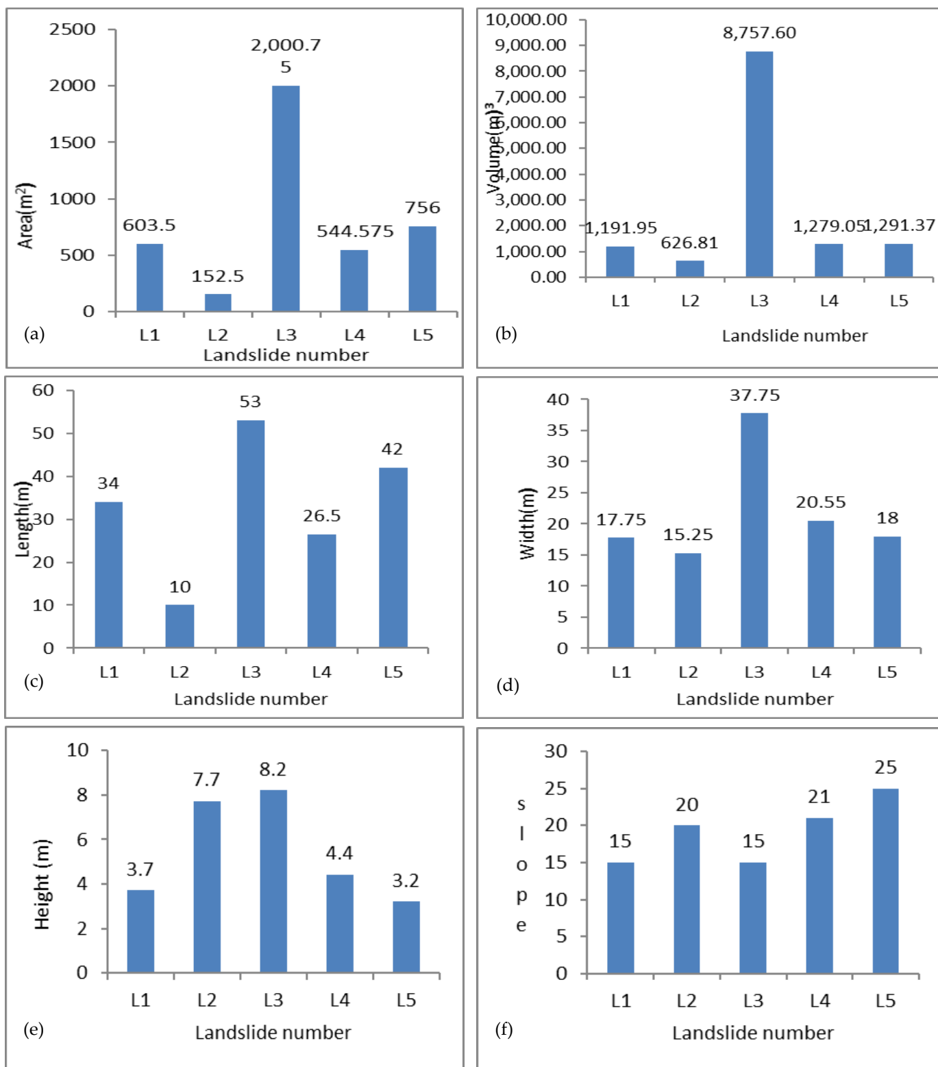
Figure 4. Plots of geometric parameters versus landslide number: (a) Area; (b) Volume; (c) Length; (d) Width; (e) Height; (f) Slope angle.
