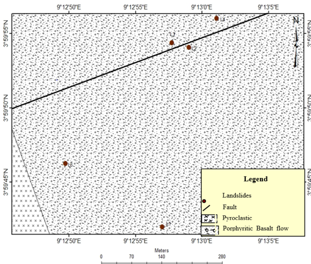
Figure 2. Geologic map of the study area.
