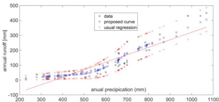
Figure 5. The proposed method with fuzzy regression curves applied in order to assess a fuzzy relation between annual precipitation and annual runoff in the case of Rio Piedras.
