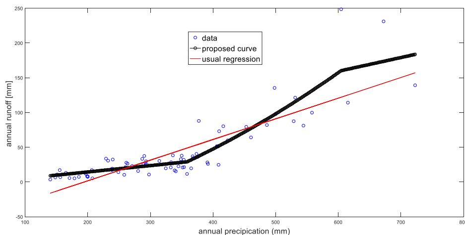
Figure 4. The proposed method and the conventional regression applied in order to assess a relation between annual precipitation and runoff in the case of Rio de Aguas.
