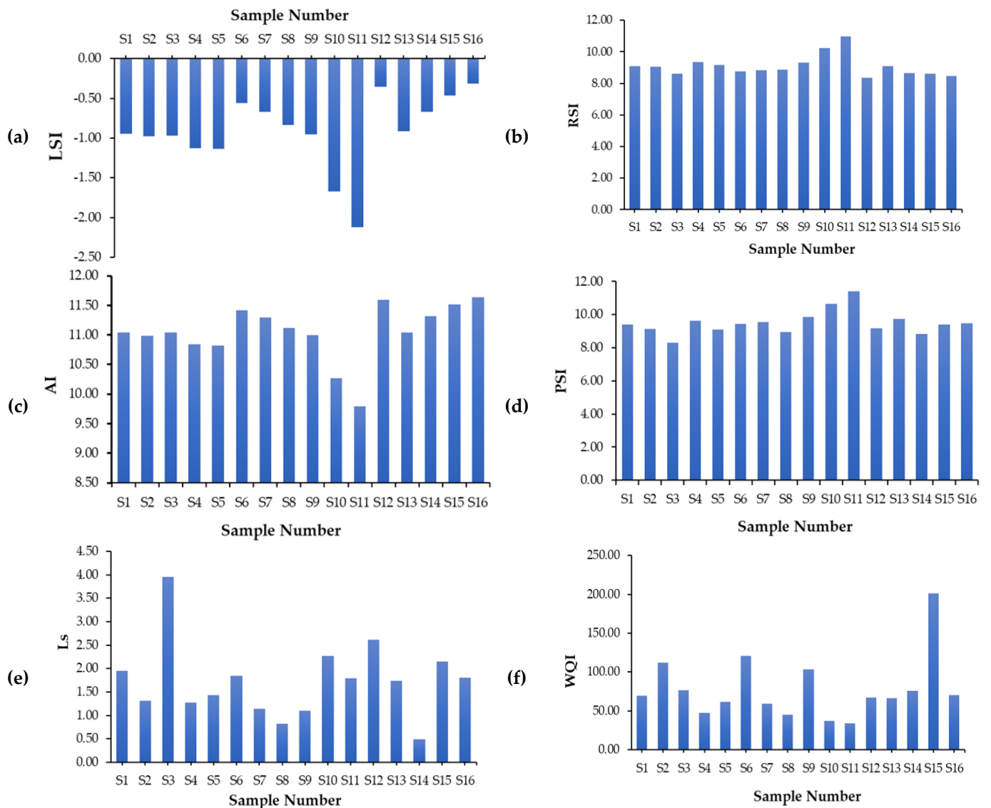
Figure 3. Corrosiveness indices and WQI of the water samples.
