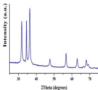
Figure 7. The XRD spectra of ZnO-NPs synthesized by biological method.
