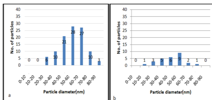
Figure 6. Histogram of size of (a) oval and (b) spherical ZnO NP that synthesized by the biological method.
