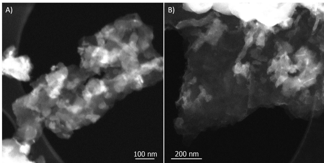
Figure 3. HADF STEM images of g-C 3 N 4 /WO 3 sample containing \omega(\text{WO}_3) = 37.5\% after hydrothermal treatment.
