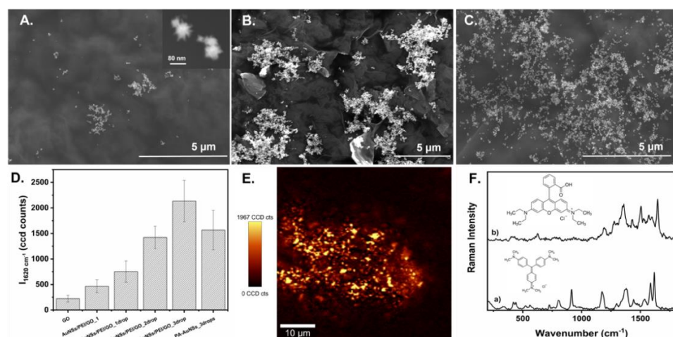
Figure 3. SEM images of AuNSs/PEI/GO_1 (A); AuNSs/PEI/GO_1drop (B) and AuNSs/PEI/GO_3drops (C); (D) Plots of the average Raman intensity of the band at 1620\text{ cm}^{-1} in the MB SERS spectrum (100 \mu\text{M} ) for GO, AuNSs/PEI/GO_1, AuNSs/PEI/GO_1drop, AuNSs/PEI/GO_2drop, AuNSs/PEI/GO_3drop, PA/AuNSs_3drop; E) Raman image obtained by integrating the area of the band at 1620\text{ cm}^{-1} of MB (100 \mu\text{M} ) using AuNSs/PEI/GO_3drop; F) SERS spectra of (a) CV (100 \mu\text{M} ) and (b) RhB (100 \mu\text{M} ) adsorbed on AuNSs/PEI/GO_3drop.
