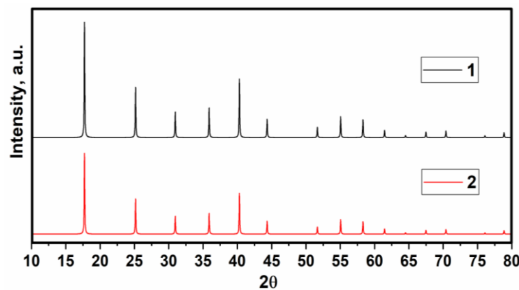
Figure 3. X-ray diffraction of nanocomposites 1 and 2 .
